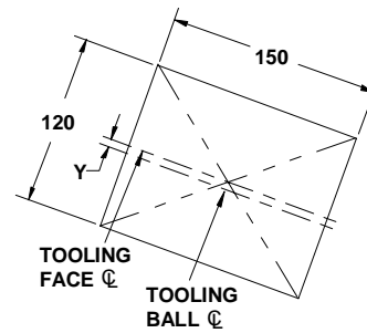
TOOLING MOUNTING FACE
