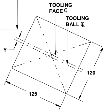
TOOLING MOUNTING FACE
